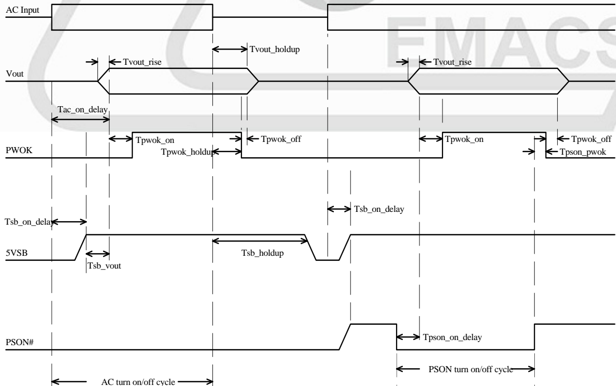
Figure 2: Turn On/Off Timing(Single Power Supply)
