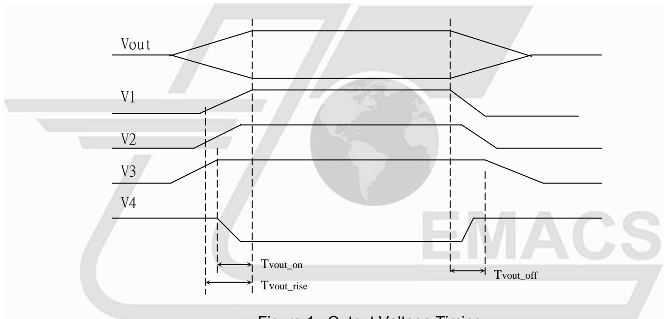
Figure 1: Output Voltage Timing
