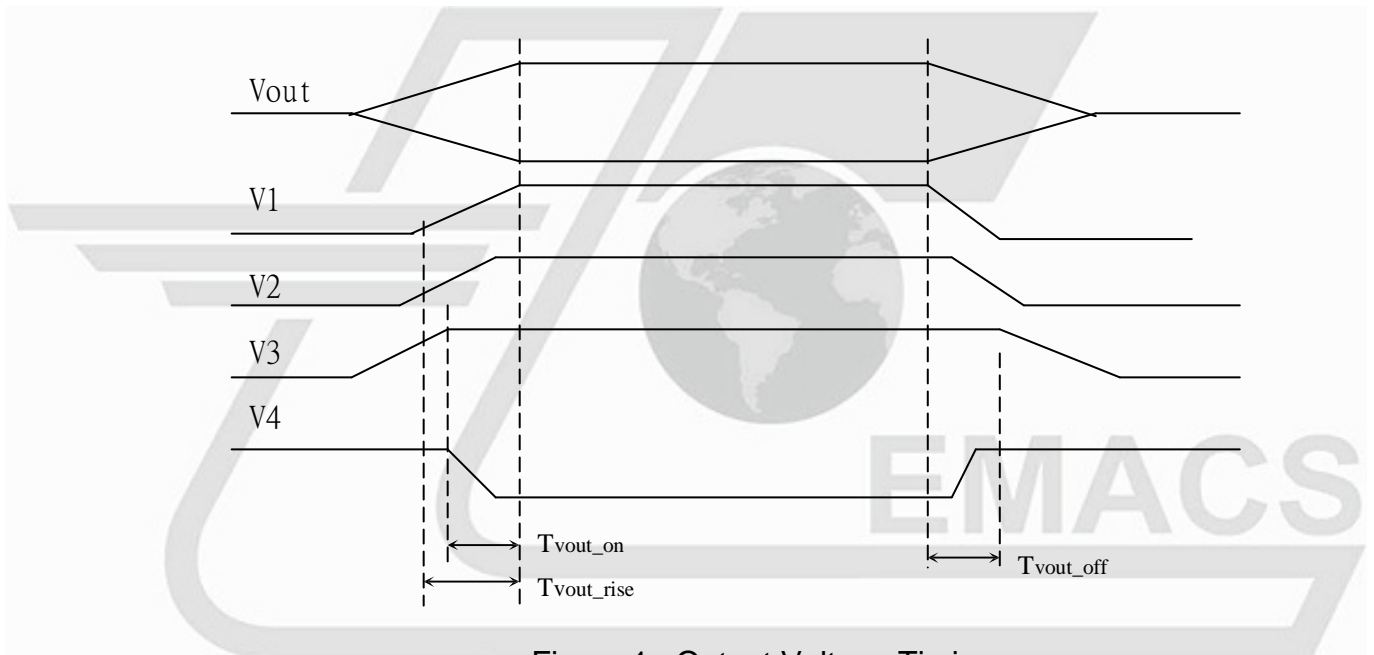
Figure 1: Output Voltage Timing
