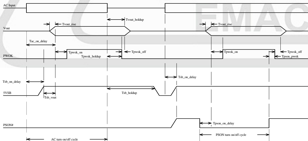
Figure 2: Turn On/Off Timing(Single Power Supply)
